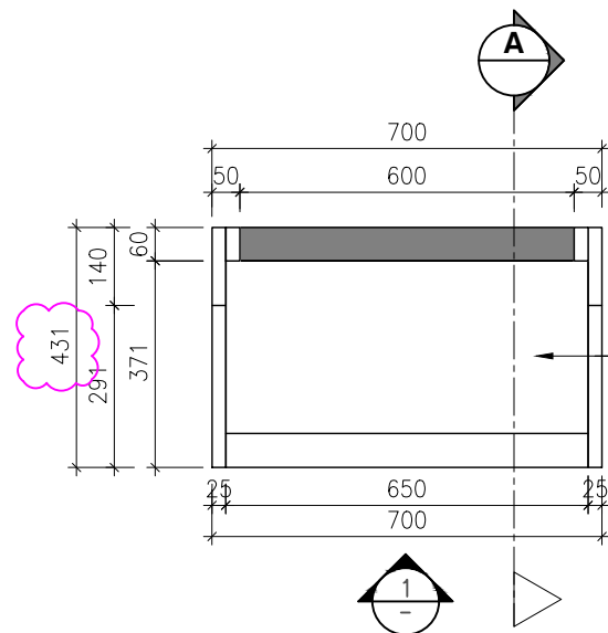
1 PLAN SCALE 1:15
