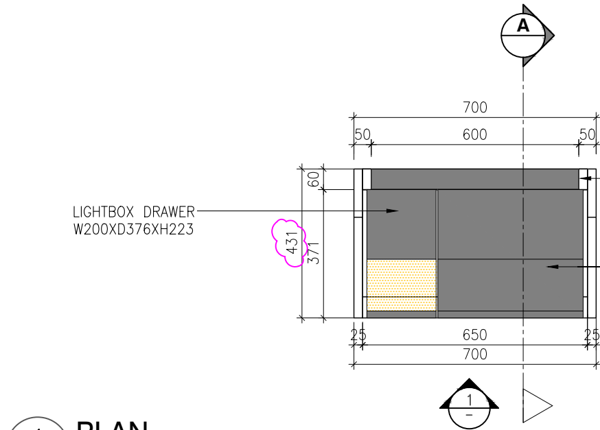
1 PLAN SCALE 1:15
