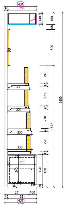
WALLBAY (STANDARD) (WB-S5)
