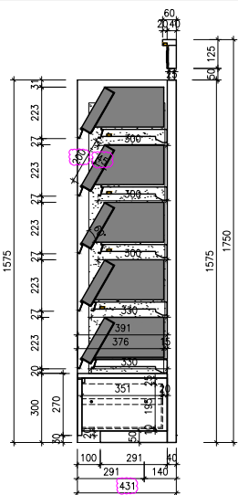
ENDCAP-BACK (MAKEUP) (EC-M)
