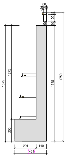
ENDCAP-FRONT (STANDARD) (EC-S)
