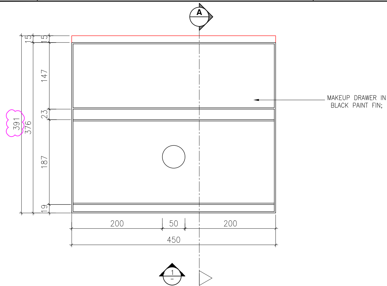
1 PLAN SCALE 1:5
