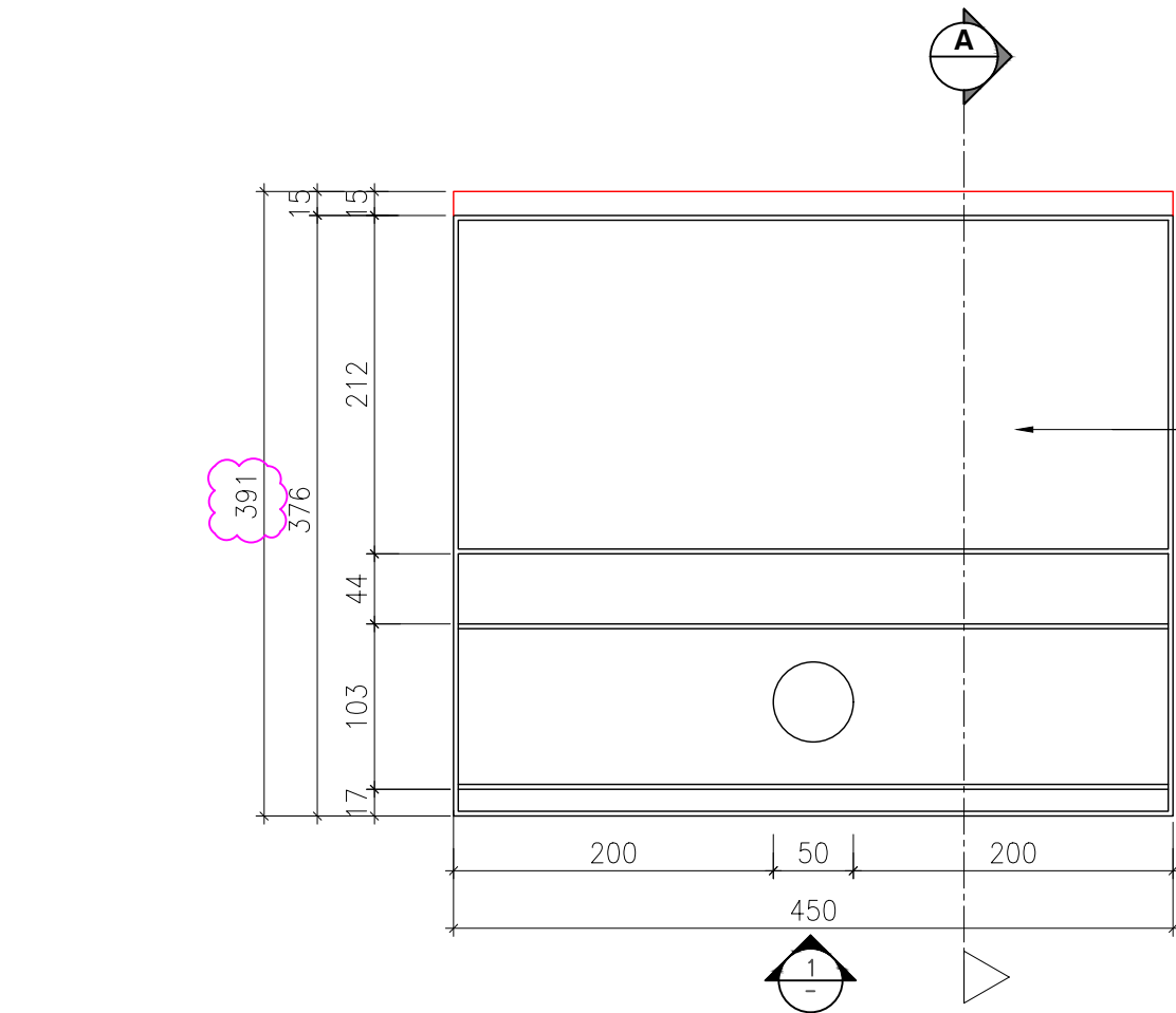
1 PLAN SCALE 1:5
