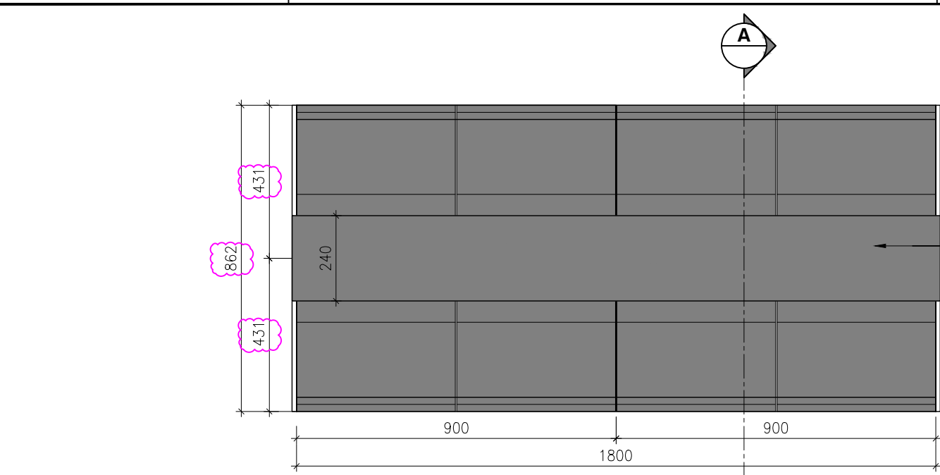
1 PLAN SCALE 1:15
