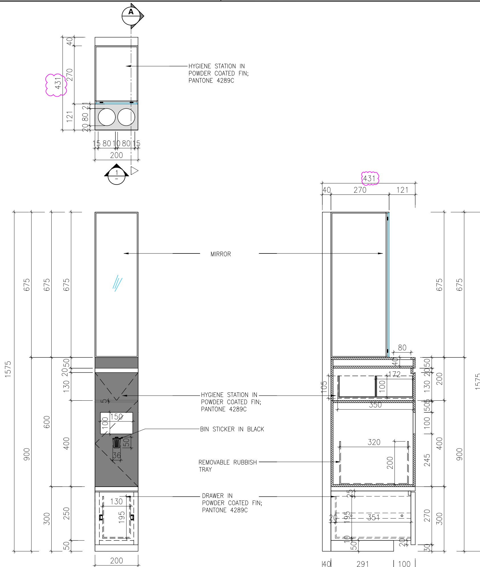
1 PLAN SCALE 1:10
