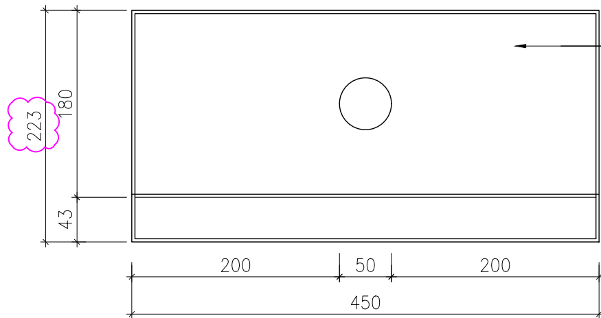
2 ELEVATION 1 SCALE 1:5
