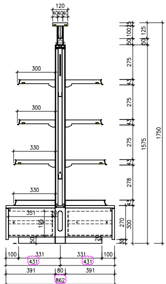
GONDOLA (STANDARD) (GD-S4)
