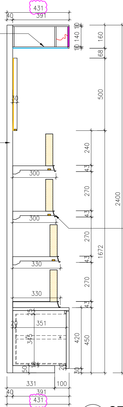
3 SECTION A SCALE 1:15
