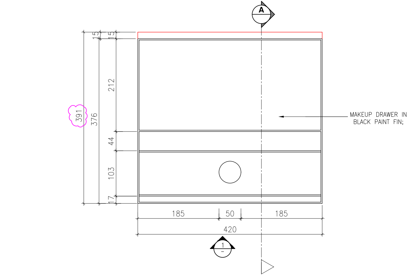
1 PLAN SCALE 1:5
