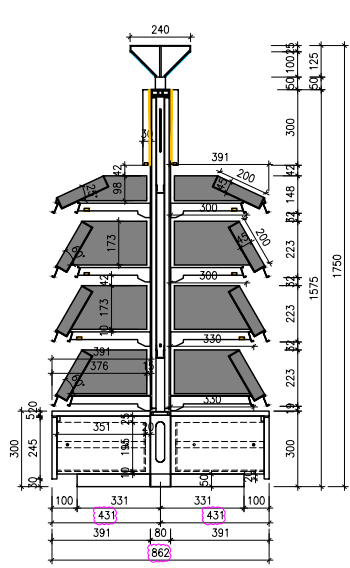
GONDOLA (STANDARD) (GD-S5)
