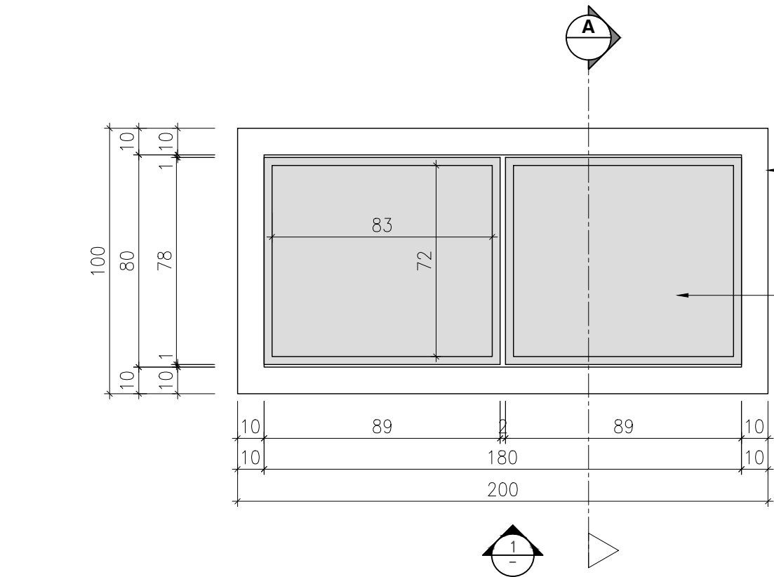
1 PLAN SCALE 1:2
