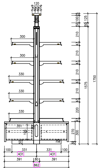
GONDOLA (MAKEUP) (GD-M)
