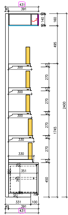
WALLBAY (STANDARD) (WB-S4)
