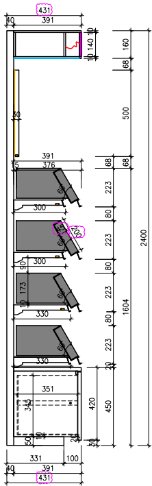
WALLBAY (MAKEUP) (WB-M)
