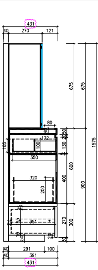
HYGIENE STATION (HS-M)
